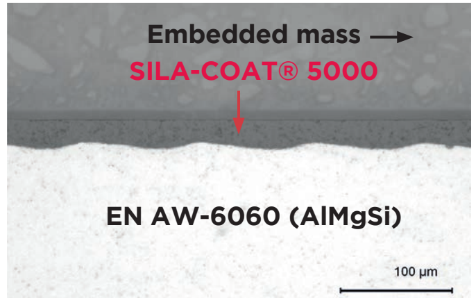
Improvement of corrosion protection and levelling of the surface with electrophoretically applied liquid paint.
