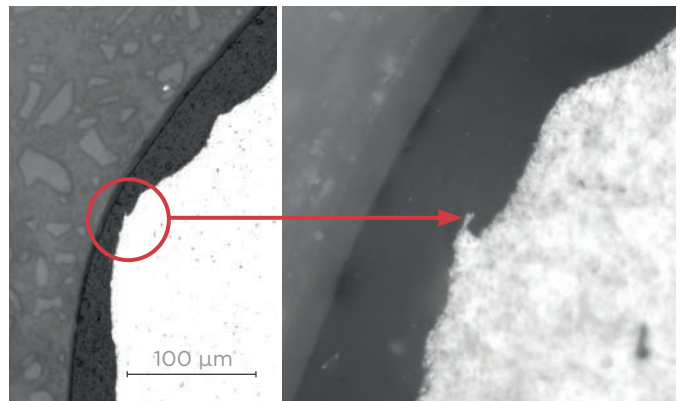
Cross section of EN AW-6060 (AlMgSi) with SILA-COAT® 5000.
