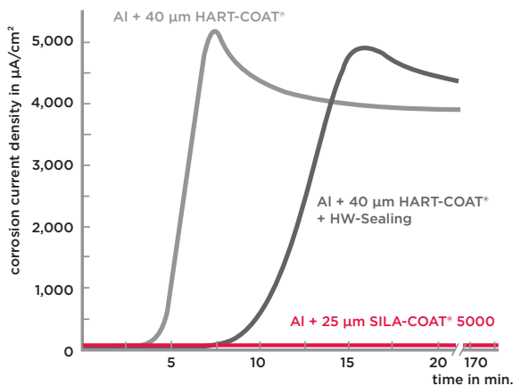
Improvement of alkali resistance compared to HART-COAT® layers. Via the chronoamperometric method (measurement at rest potential) it can be determined after which time the corrosion attack starts. In this case the measurement was performed in a 3 % aqueous sodium hydroxide solution.
